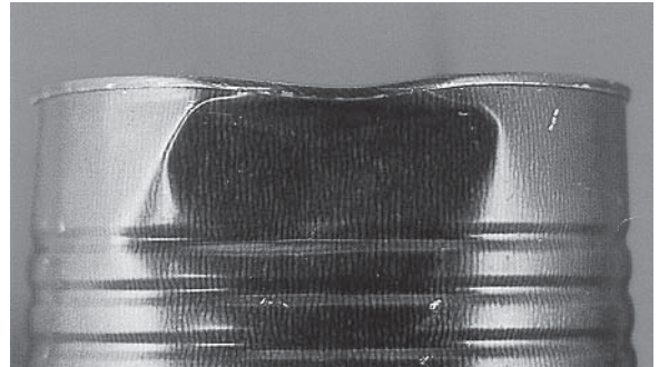
2 Severe body dent has affected double seam. Observe for fractured plate.
