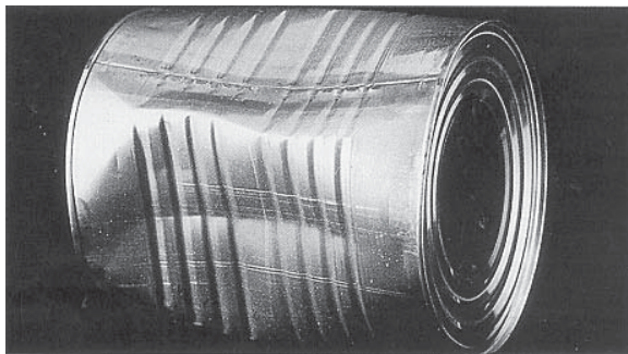
3 Paneled, beaded can. Materially affecting appearance, but not integrity, i.e. no plate fractures.
