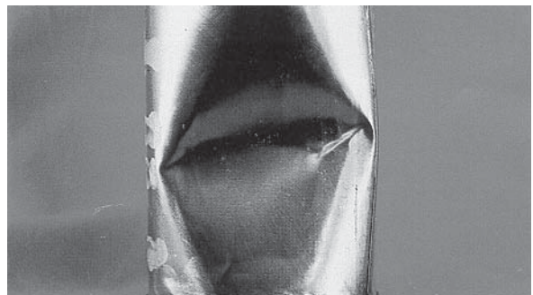
2 Severe body dent. Observe for fractured plate.
